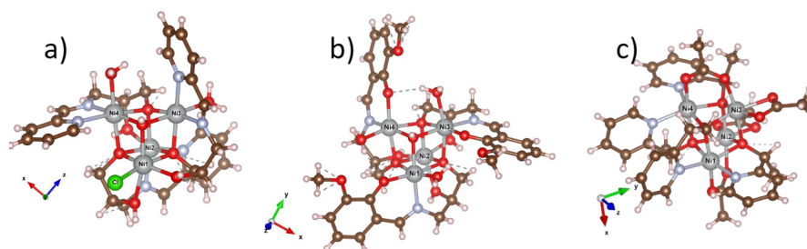
Fig. 1: Ni 4 complexes studied: a) [Ni 4 (...) 3 (Cl)(μ 3 -OH)(H 2 O) 2 ], b) [Ni 4 (...) 3 (μ 3 -OH)(H 2 O) 2 ], c) [Ni 4 (...) 4 (CH 3 COO) 4 ], where red – oxygen; brown – carbon; white – hydrogen; grey – nickel; purple – nitrogen; green – chlorine.
